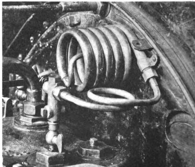
Maxim Tire Inflation Apparatus Is Very Simple.
